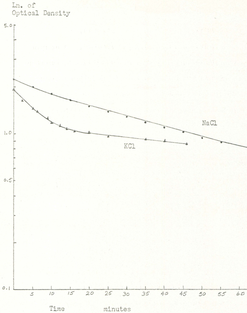
Figure 13. Plot of natural logarithm of optical density as a function of time. Illumination with white light.
