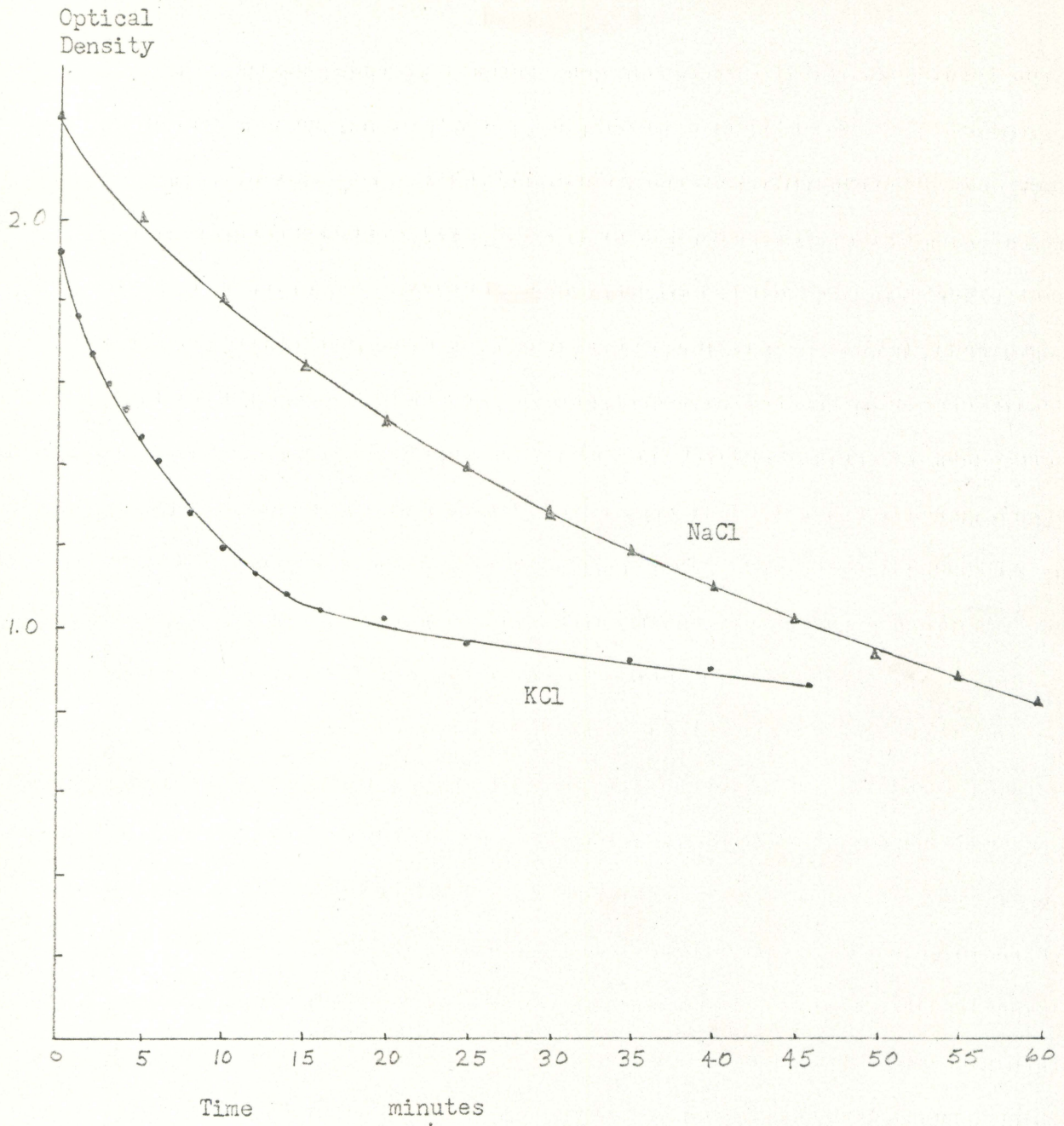
Figure 12. Decay of F-center peak illuminated with white light.
