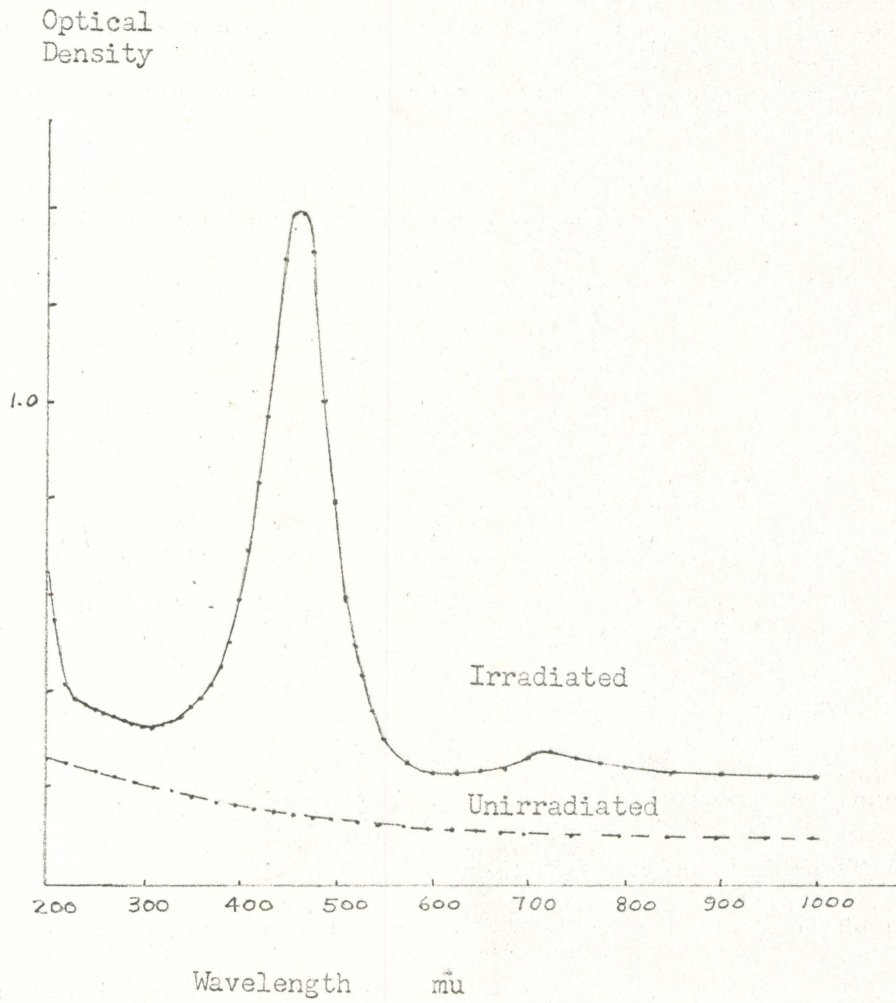
Figure 4. Optical density as a function of wavelength in NaCl.
