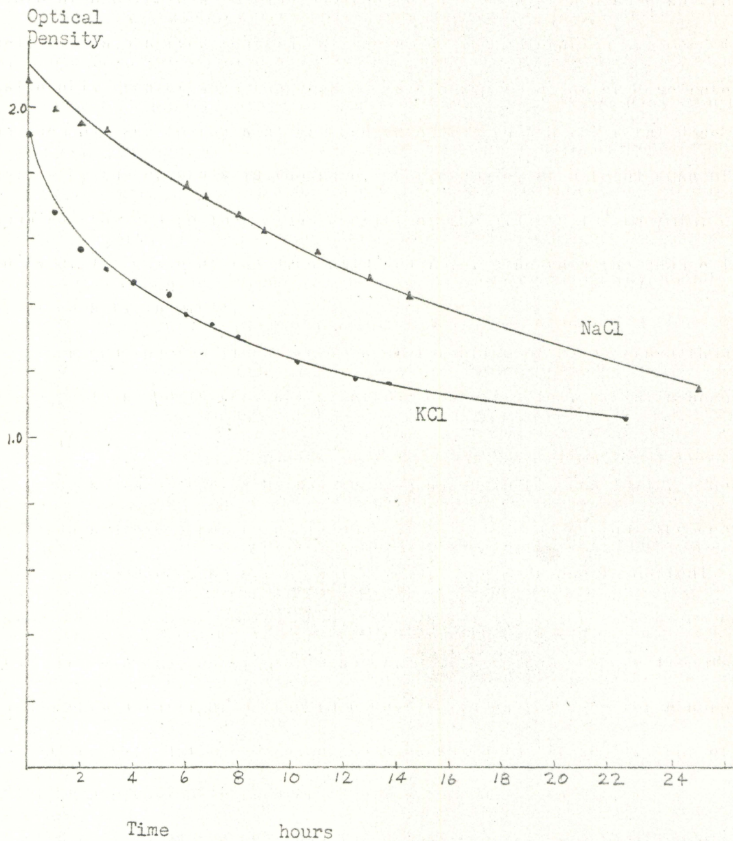
Figure 11. Decay of F-center peak illuminated with F-light.
