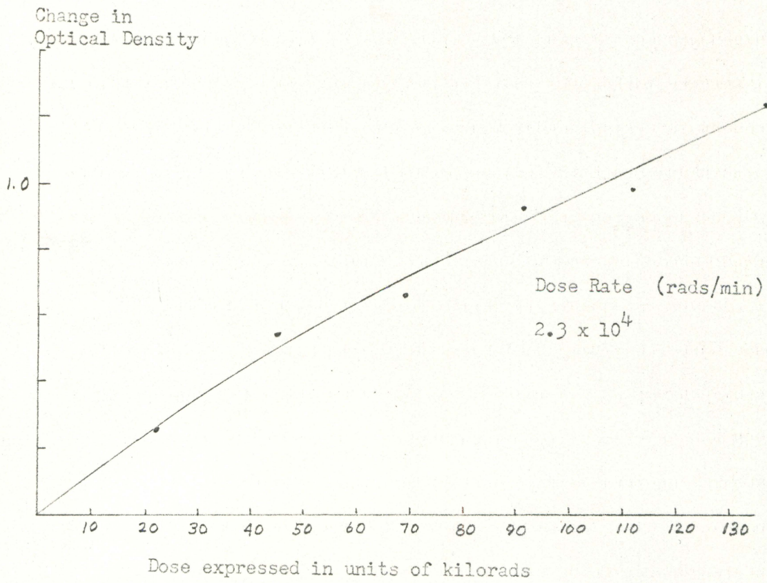
Figure 9. Change in optical density as a function of irradiation dose in LiF.
