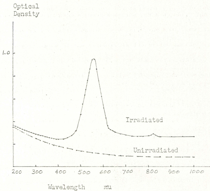
Figure 5. Optical density as a function of wavelength in KCl.
