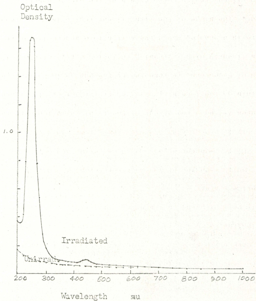
Figure 6. Optical density as a function of wavelength in LiF.
