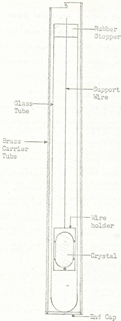
Figure 3. Schematic diagram of crystal mounting arrangement.
