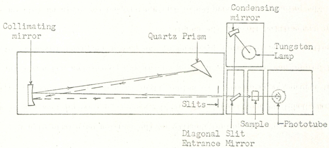
Figure 1. Diagram of spectrophotometer optical path.
