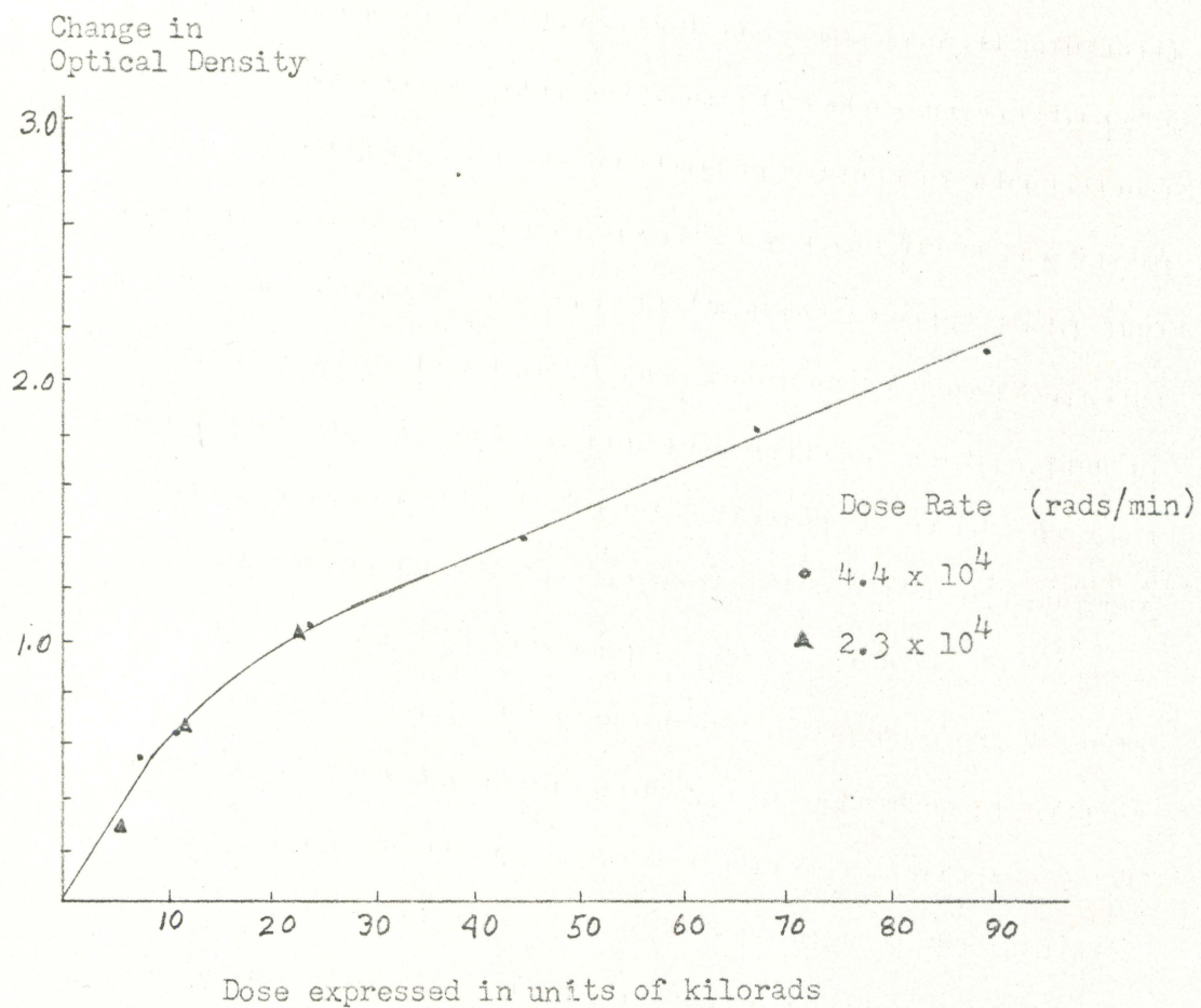
Figure 7. Change in optical density as a function of irradiation dose in NaCl.
