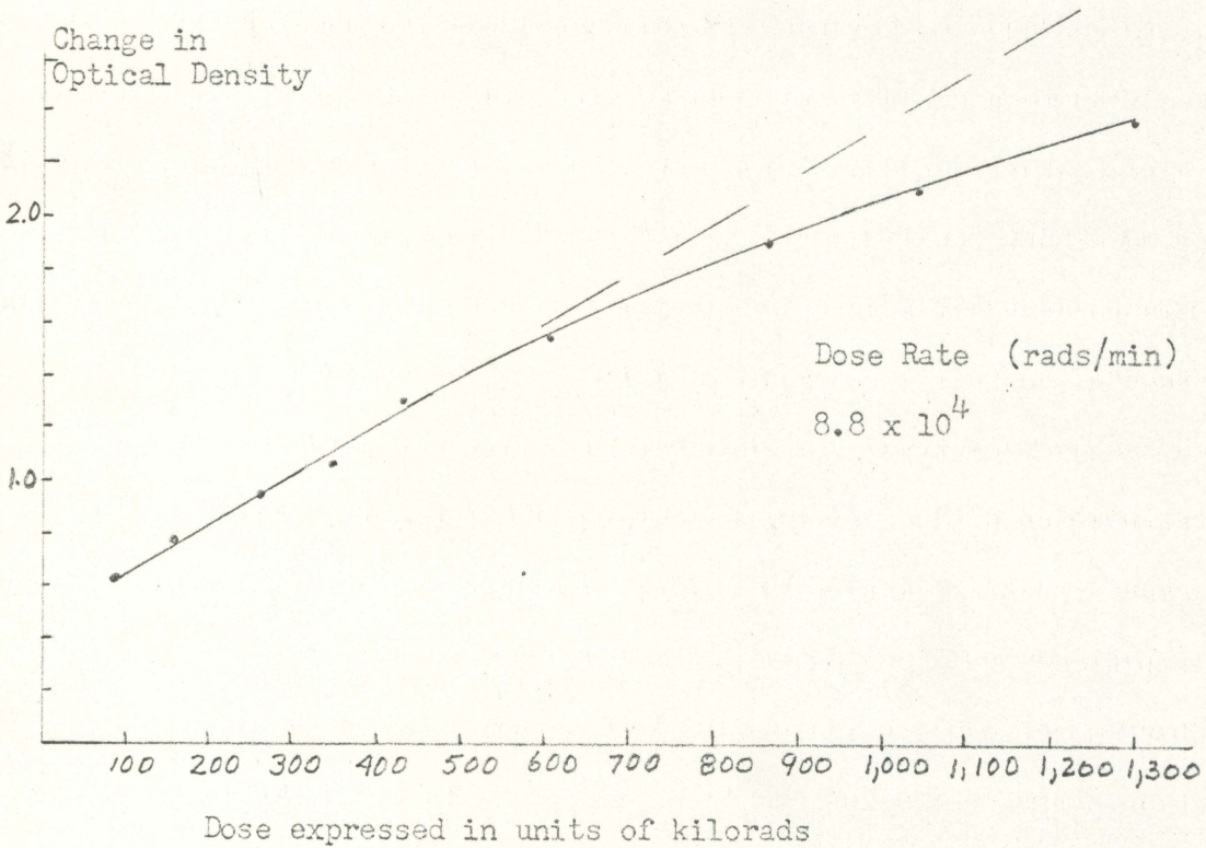
Figure 8. Change in optical density as a function of irradiation dose in KCl.
