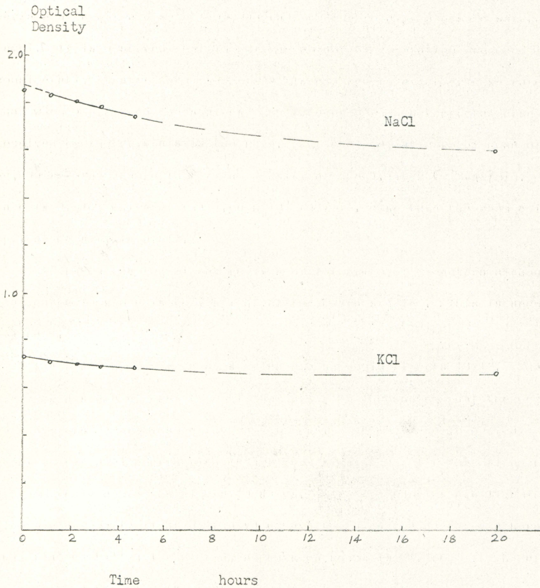
Figure 10. Decay of F-center peak with no illumination.
