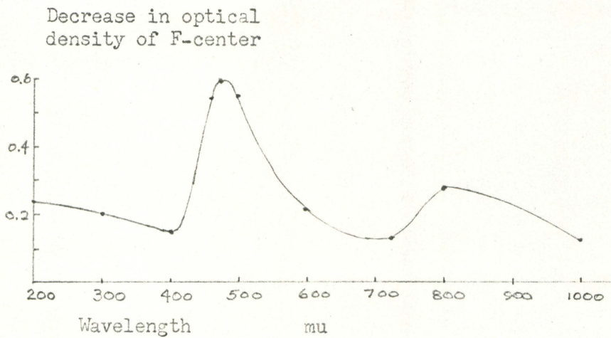
Figure 14. Comparison of decrease in F-center peak and change in M-center peak as a function of the wavelength of illuminating or bleaching light.
